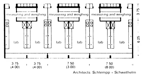
② Uniform labs with measuring and weighing rooms in front of them (University clinic in Frankfurt/Main)
